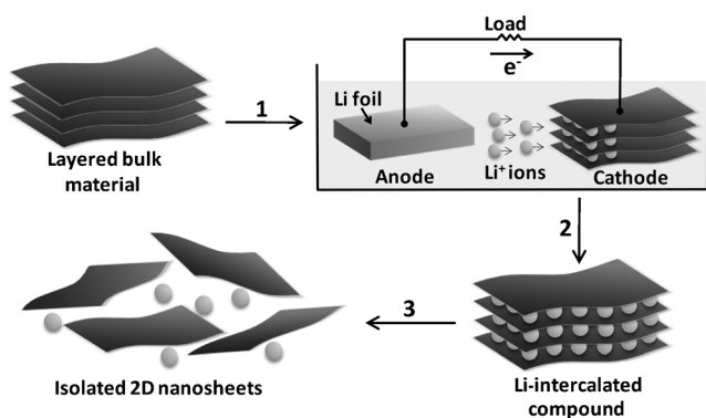
Figure 1. Electrochemical lithiation process for the fabrication of 2D nanosheets from the layered bulk material.
